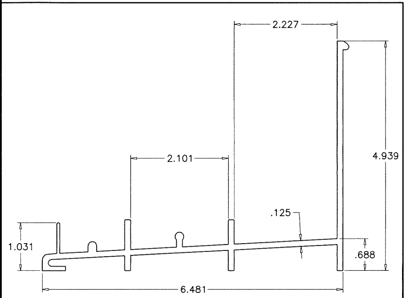
2 FRAME SILL (4-15/16")
