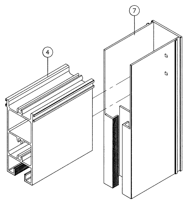
PANEL CORNER
