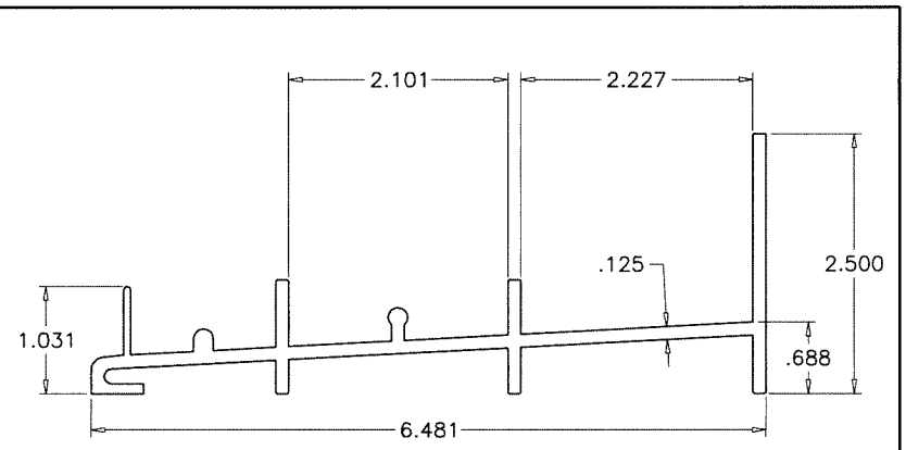
2C FRAME SILL (2-1/2")
