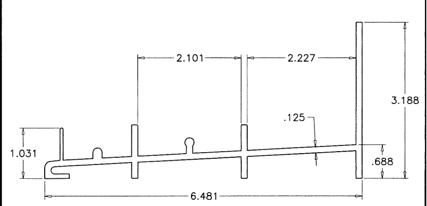
2B FRAME SILL (3-3/16")
