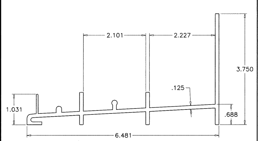
2A FRAME SILL (3-3/4")
